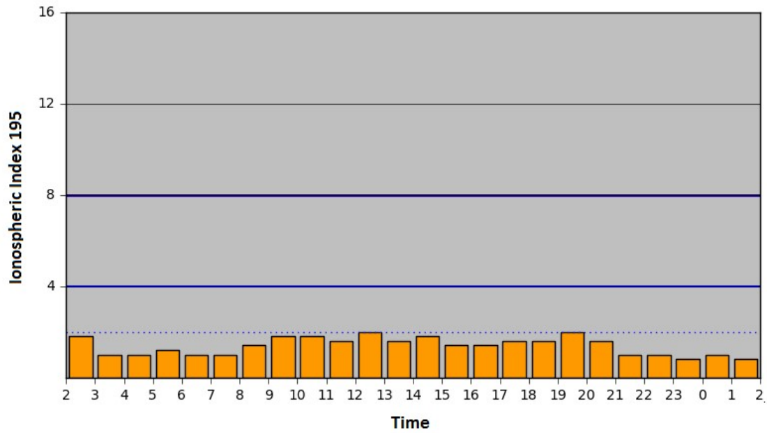
Figure 4.2 Ionospheric noise 195 index, first 14 th of September; second 16 th of September. The line with the dots (2) means undisturbed, blue line (4) means a light disturbance and the dark blue line (8) means a high disturbance.
