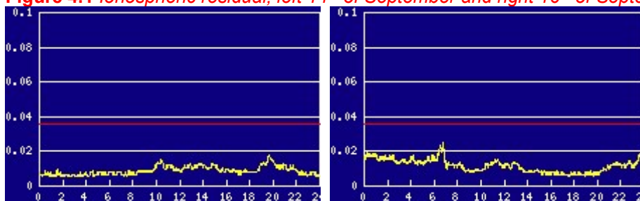
Figure 4.1 Ionospheric residual, left 14 th of September and right 16 th of September.
