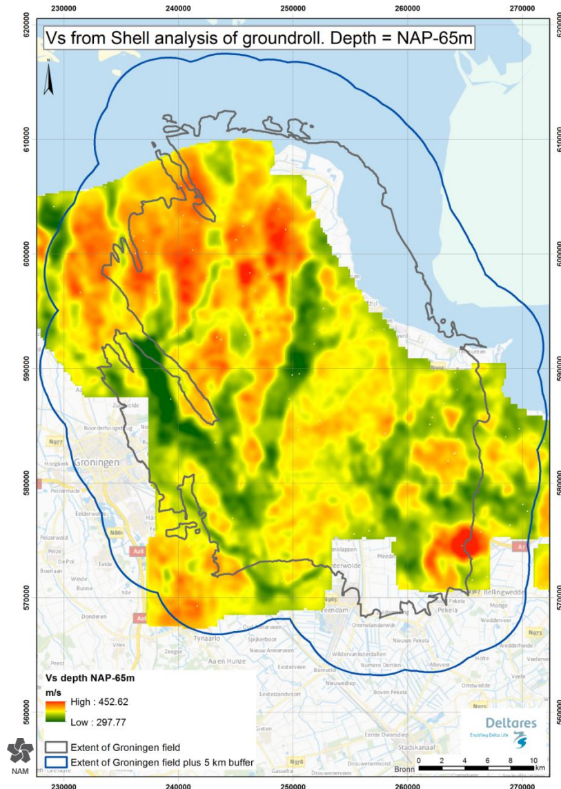
Figure 3.43 The V_s model from the inversion of the ground roll yielded depth slices of V_s at 10 m depth intervals. This figure shows a depth slice at NAP-65 m through the MEIDAS V_s model.
