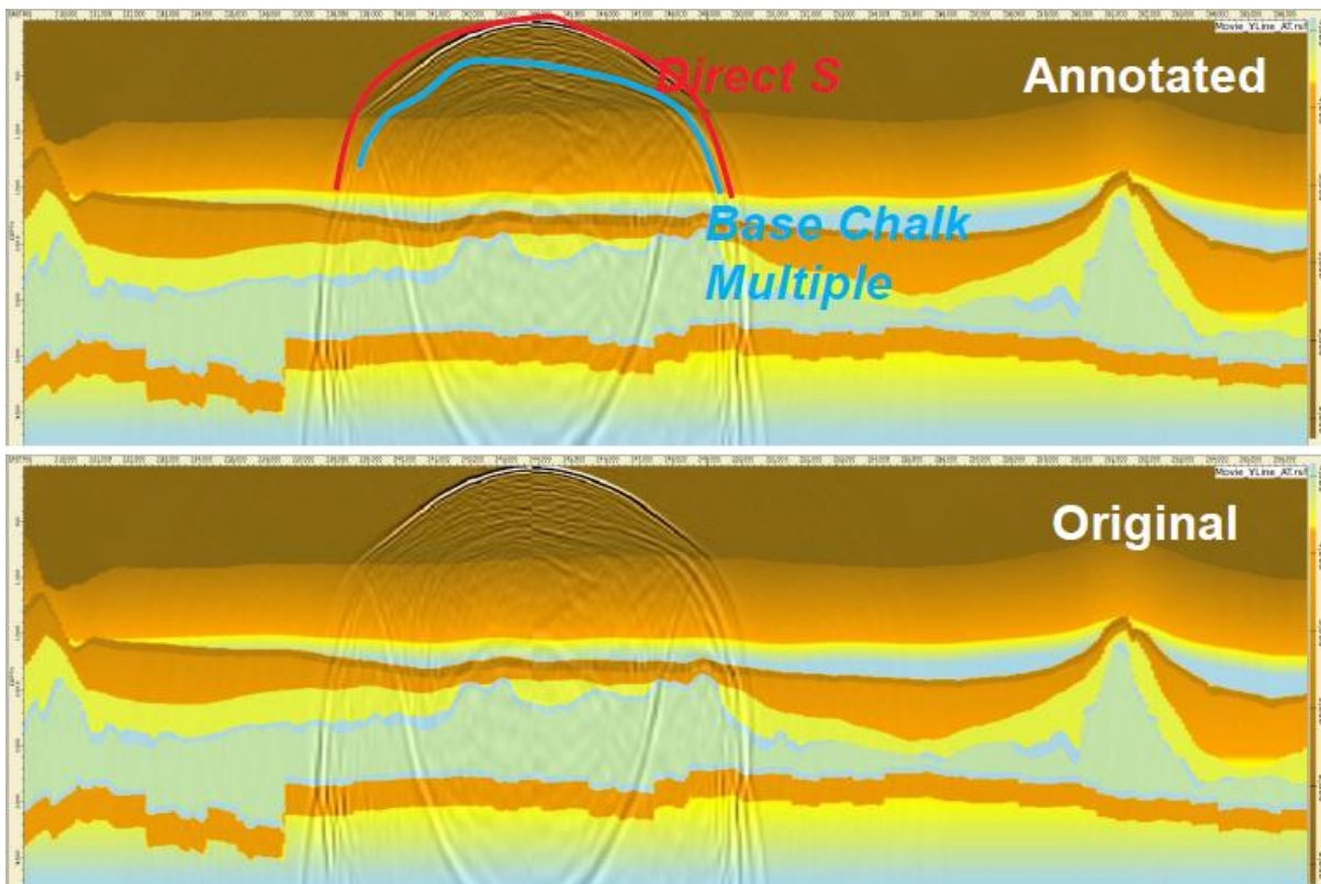
Figure 3.40 Image of the modelling of the progression of the seismic waves from the rupture area in the reservoir to the surface. This modelling does not include the effects of the approximately 350 m deep soil layer. The snapshot was taken 2.7 seconds after the rupture took place, when the S-waves reaches the surface.
