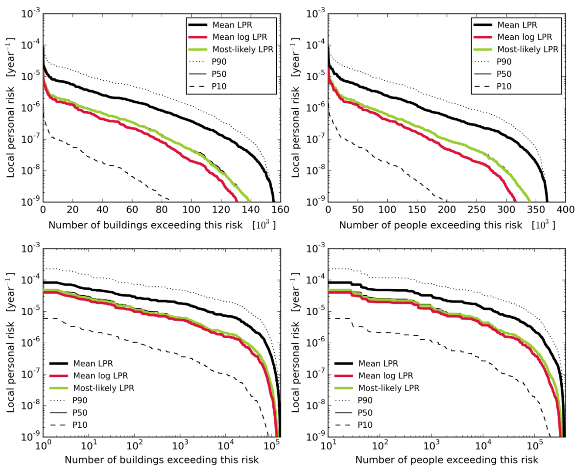
Figure 6.2 Number of buildings and people exceeding a given inside local personal risk shown on (top) a linear scale for the overall view and (bottom) a log scale to accentuate the lower end of the building count. These figures are for the 33 bcm/year production scenario and the 2016-2021 assessment period.
