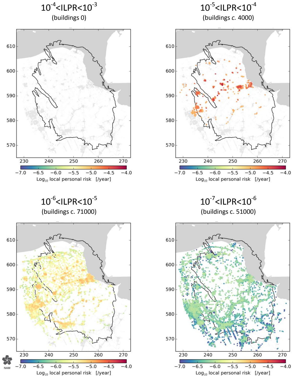
Figure 6.5 Mean inside local personal risk, ILPR for every individual building within four equal risk bands from 10^{-7} to 10^{-4} /year for the 5-year assessment period 2016 to 2021 under the 33 bcm production scenario without structural upgrading.
