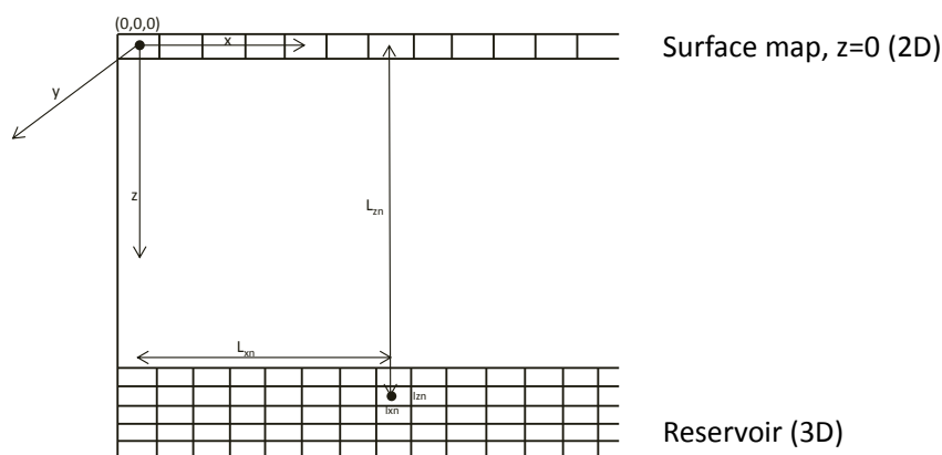
Figure A.1 Subsidence modelling schematic
