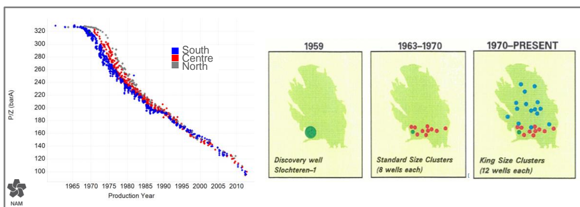
Figure 2.1 Phased development of Groningen field and historical pressures. This pressure data is available on Feiten en Cijfers at www.namplatform.nl .
