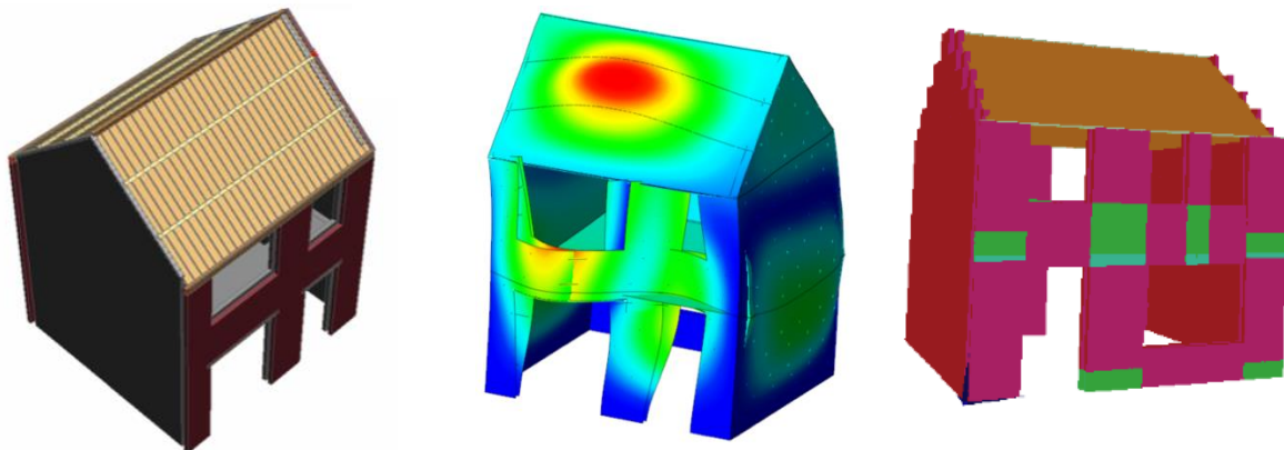
Figure 5.15. Numerical models (developed by Arup, TU Delft, Eucentre) of full-scale terraced house building tested on the shaking table
