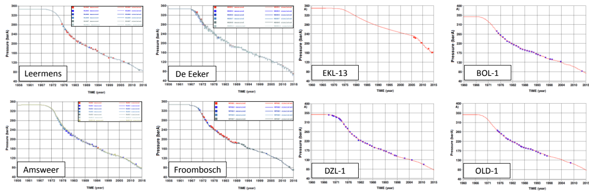
Figure 3.6 Reservoir pressure history match quality for a few typical Groningen clusters, Eemskanaal 13 and some observation wells
