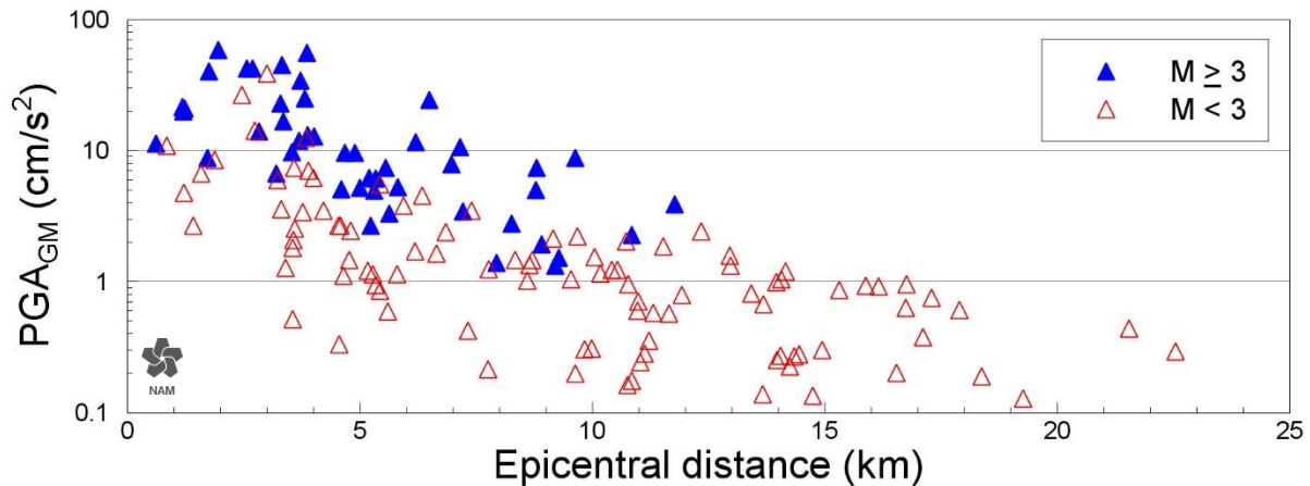
Figure 3.36. Geometric mean values of horizontal PGA plotted against epicentral distance. General trends of increasing acceleration with increasing magnitude and decreasing distance can be observed, as would be expected. A noteworthy observation is that less than 30 records (i.e., about 20% of the dataset) have geometric mean PGA values greater than 0.01g.
