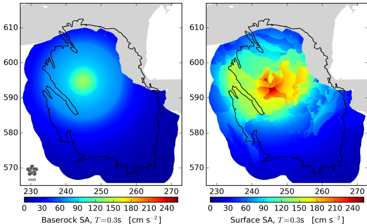
Figure 4.9 Ground motion spectral acceleration (SA) prediction. Example for M = 5
