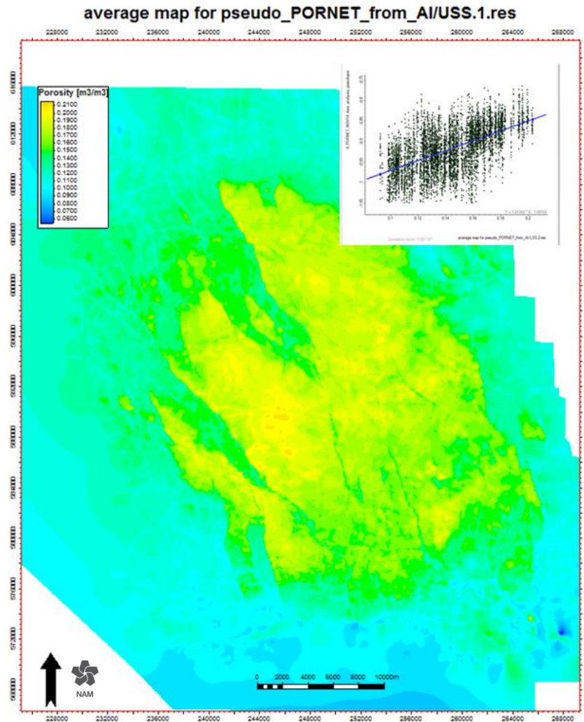
Figure 3.4 USS.1.res pseudo porosity average map has a good correlation coefficient with Net porosity and can be used for populating the 3D grid away from well control.
