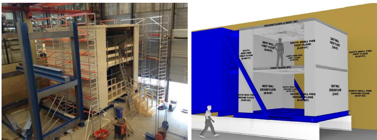
Figure 5.17 Wall and floor assemblage built in Technical University Delft.
