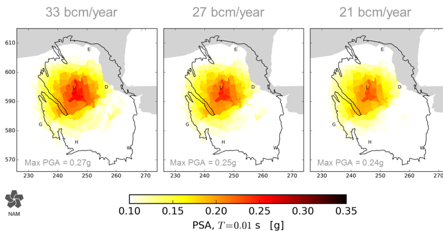
Figure 4.14 Mean PGA hazard sensitivity to production rates. Period: 2016/1 – 2021/1, Production scenarios: 33, 27, 21 bcm/year, Compaction: Inversion-linear, Seismological model: V2, M \geq 3.5 , GMPE: V2 Metric: 0.2% year -1 chance of exceedance (equivalent to 10% chance in 50 years)
