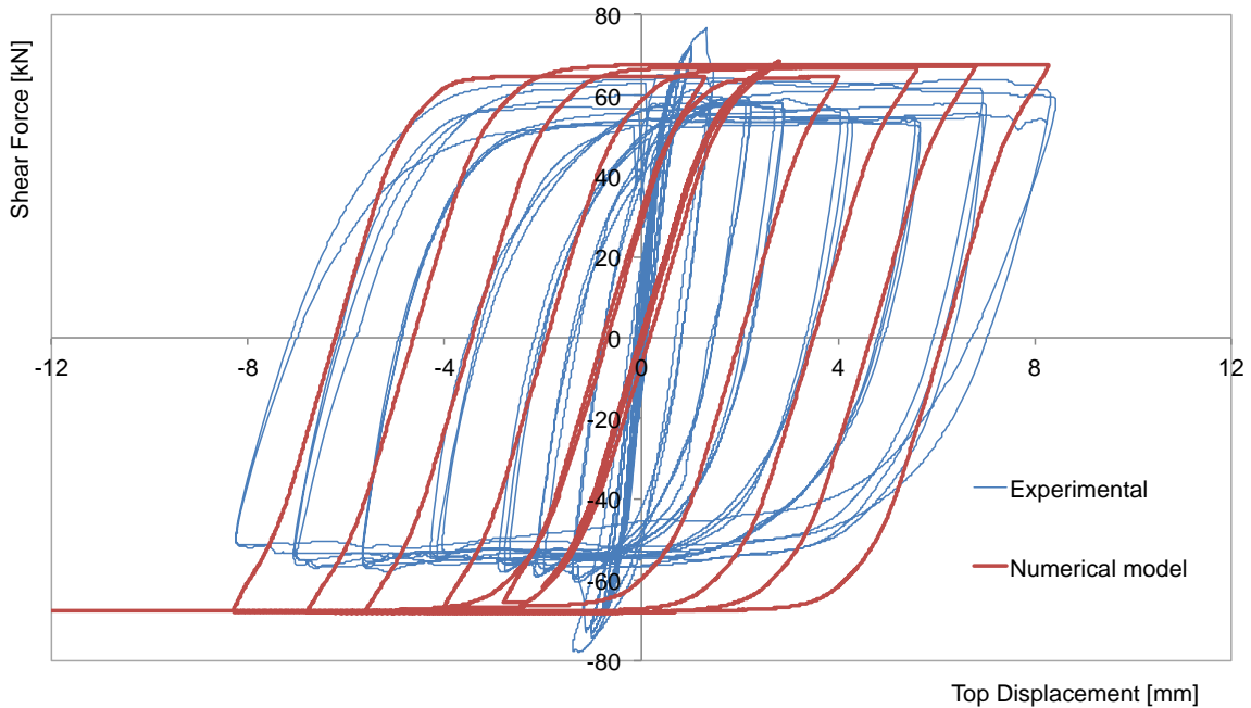
Figure 5.12 Example comparison of experimental in-plane response of calcium silicate wall and predictions by one of the modelling teams.
