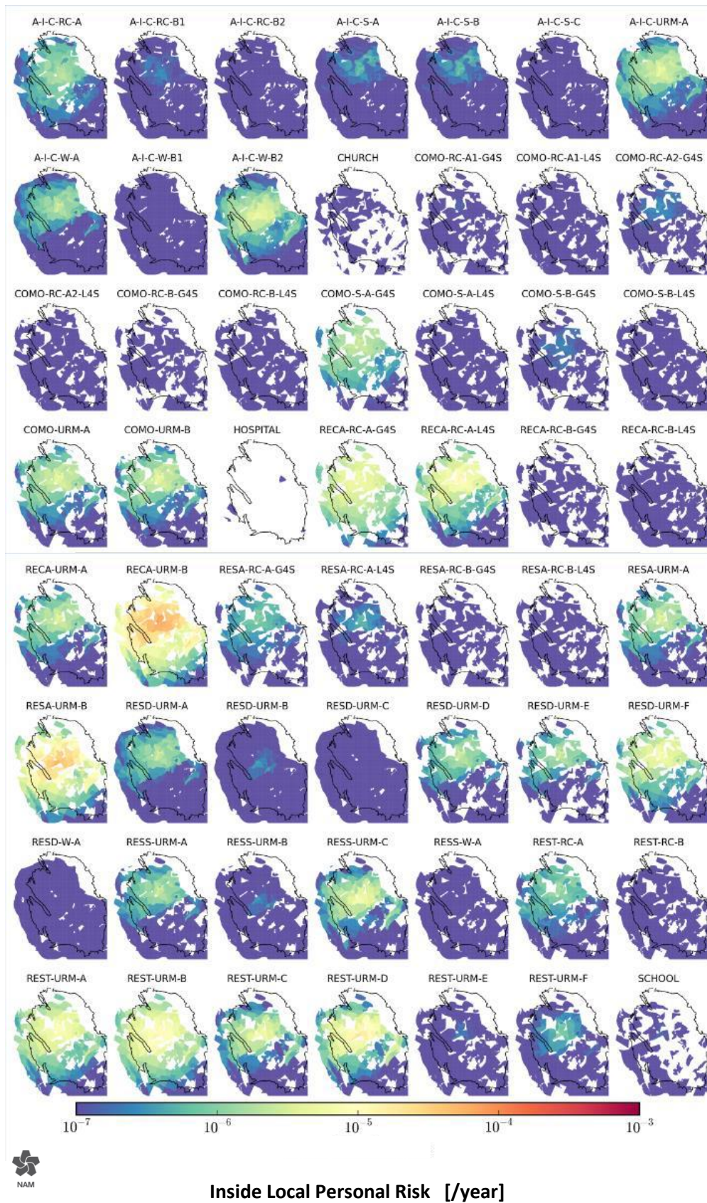
Figure 6.4 Maps of inside local personal risk according to building typology under the base-case risk assessment for the period from 2016 to 2021.
