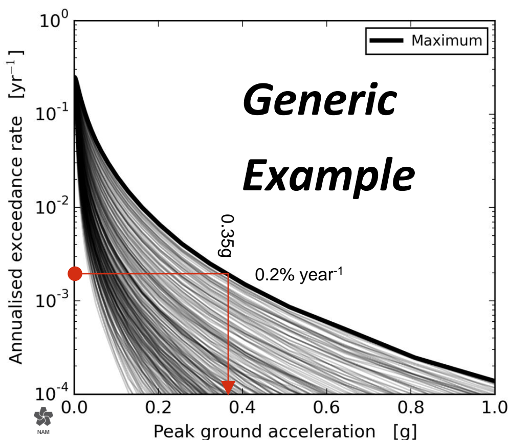
Figure 4.2 A generic example of a set of hazard curves showing average annual exceedance rate for peak ground acceleration at different locations in the field. Each line corresponds to a location in the field. The bold line indicates the maximum PGA anywhere within the field for a given exceedance level (bounding envelope). In this generic example, the red line indicates that for an exceedance level of 0.2%/year the highest PGA in the field is 0.35g.
