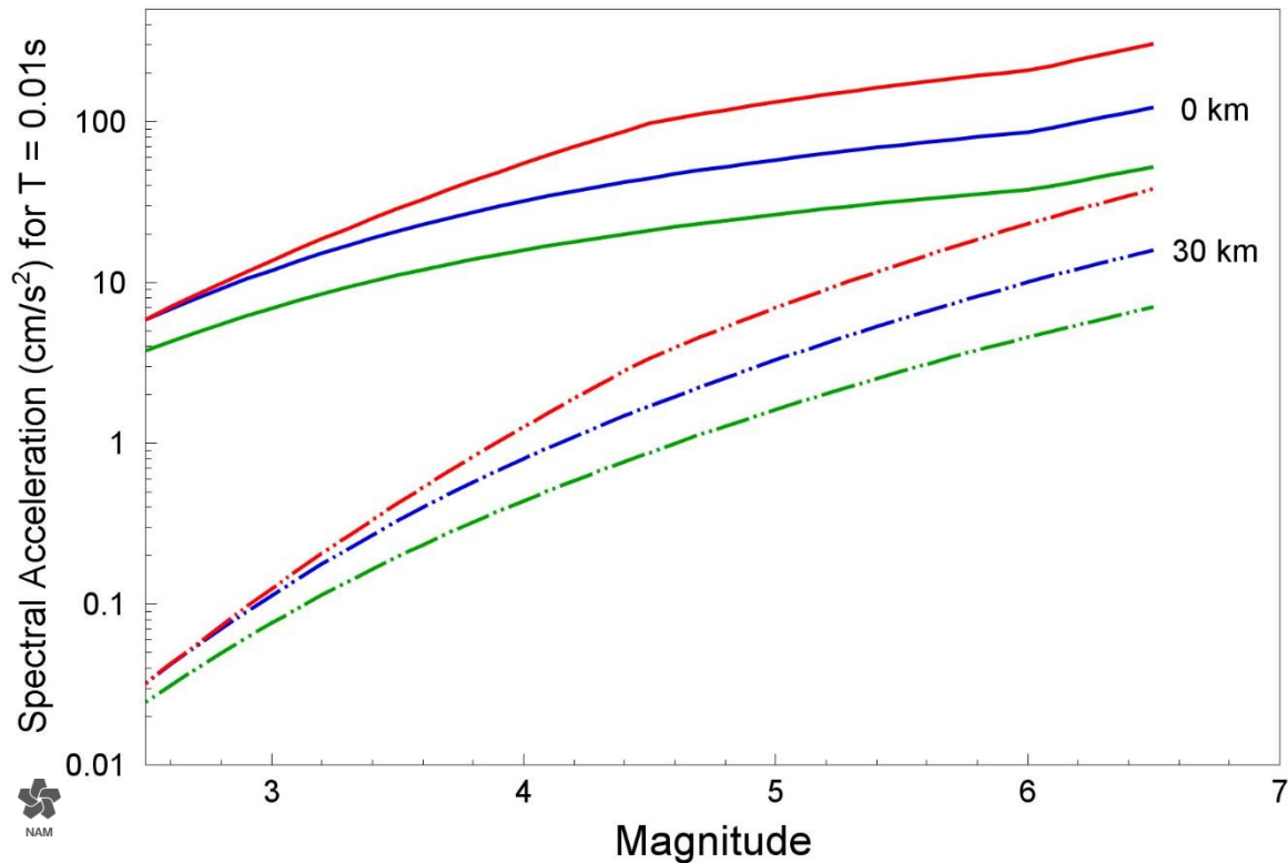
Figure 3.41. Spectral accelerations at 0.01 s from point-source stochastic simulations for lower (green), central (blue) and upper (red) models at epicentral distances of 0 and 30 km as a function of magnitude
