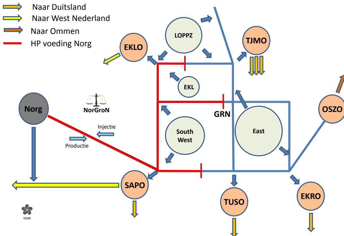
Figure 3.19 Schematic of the Groningen gas ring pipeline system as operated during the summer months with two pressure regimes.
