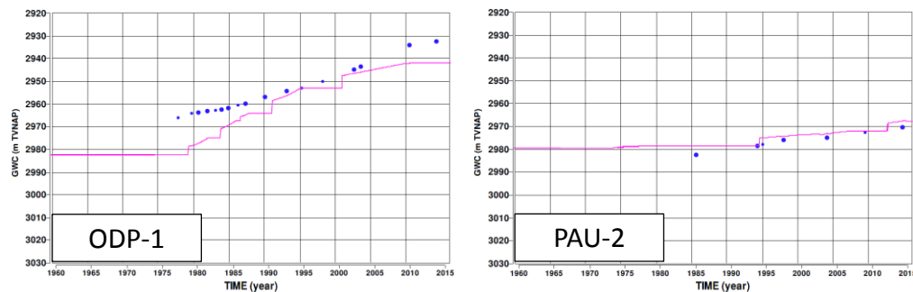
Figure 3.18 History match quality on water rise (PNL) using some example wells.
