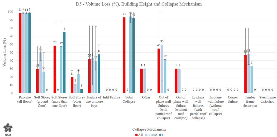
Figure 5.29 Distribution of volume loss by collapse mechanism and height for collapsed buildings based on observations (So et al., 2015)
