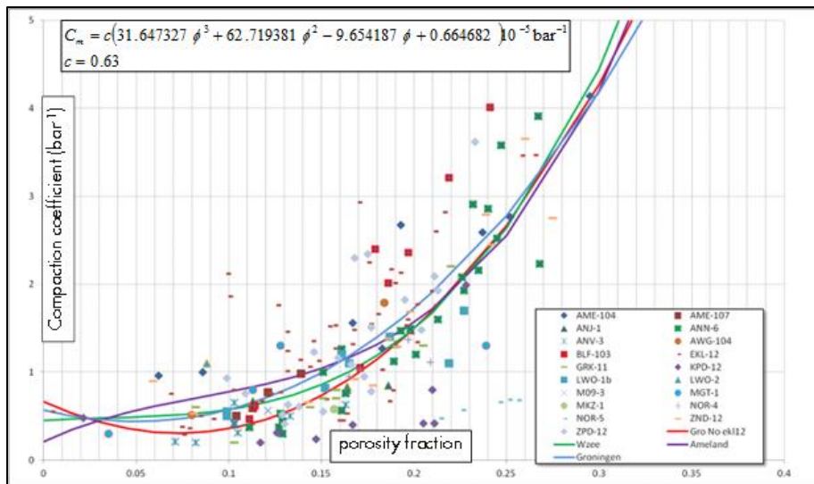
Figure A.9 Compressibility coefficient relation versus porosity based on first cycle cm core data, from Ref [5][5]. The constant which has been used in the GFR2012 models is c=0.55 instead of the c=0.63 as noted in the plot
