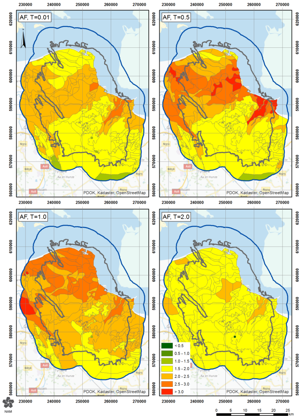
Figure 3.44 Amplification factors (AF) for the Groningen region for a scenario with M 4.0 and R_{epi} 50 km. AF for four periods are shown.
