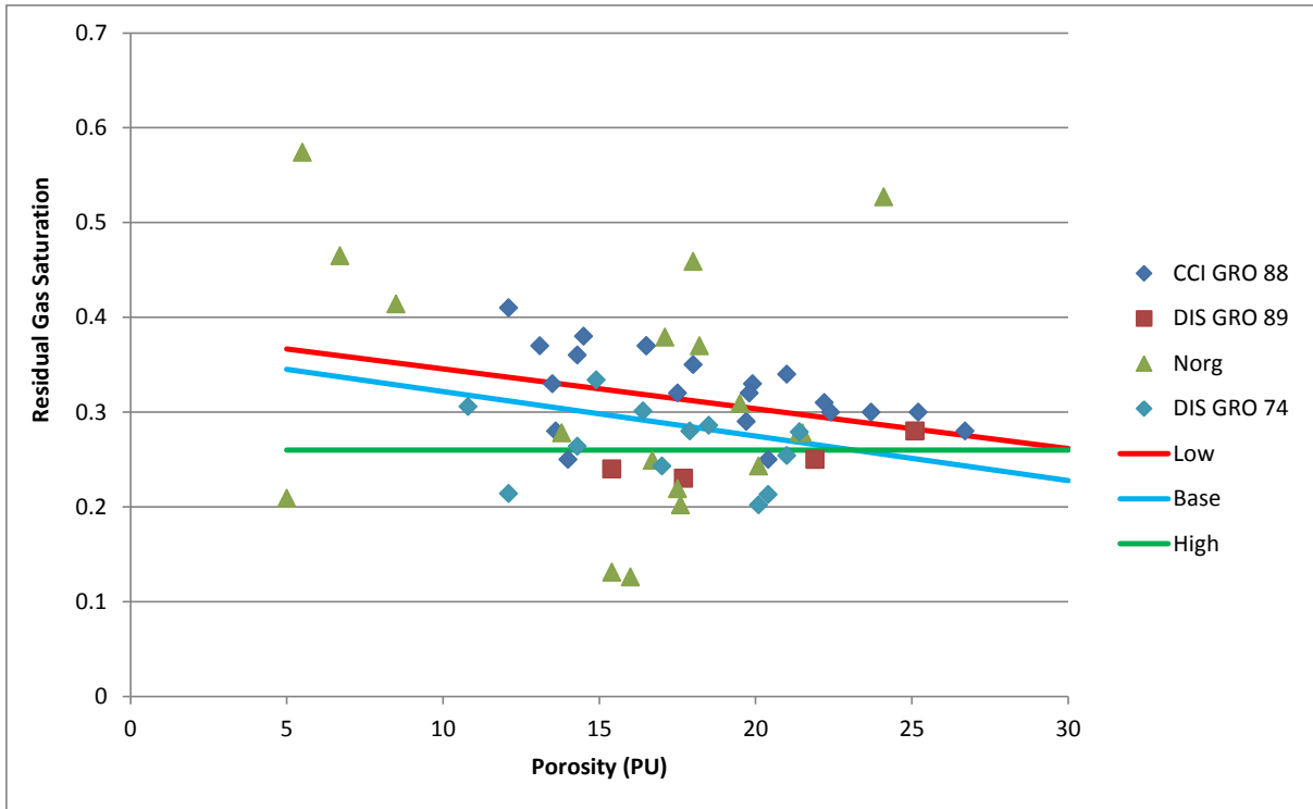
Figure A.5 S_{gr} dependence on porosity for Low, Mid and High cases.
