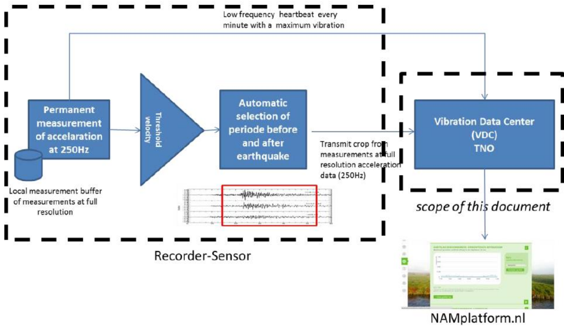
Figure 5.7 Data transfer from vibration monitoring system to Vibration Data Center (VDC)
