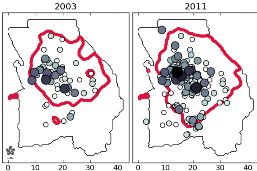
Figure 3.30 The areal extent of M \geq 1.5 earthquake locations through time remains for the most part (80%) within the 0.18 m reservoir compaction contour (red line) according to the linear poroelastic reservoir compaction model.
