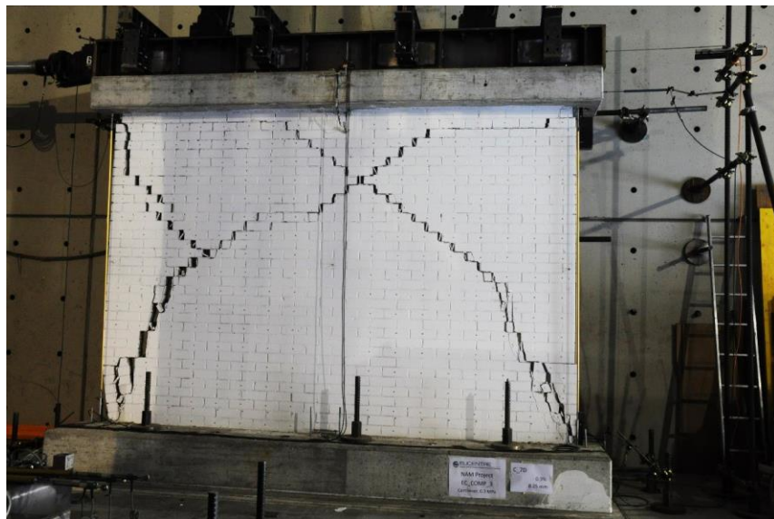
Figure 5.11 Masonry walls constructed by Groningen masons and tested in laboratories (EUCentre et al., 2015).
