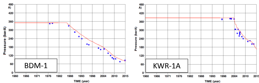
Figure 3.7 Reservoir pressure history match quality of some wells drilled in smaller fields located around the Groningen field.
