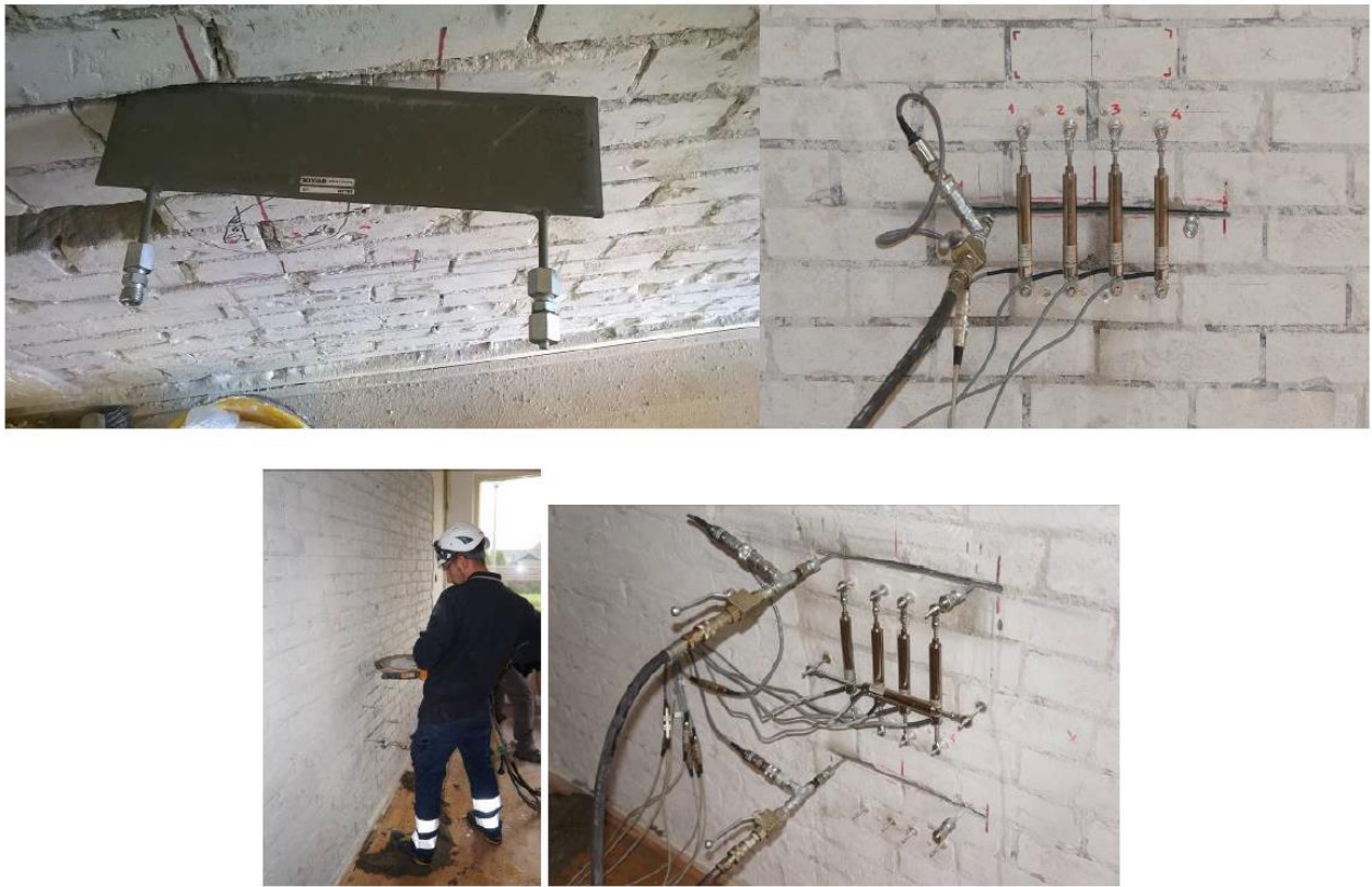
Figure 5.10 In-situ material tests on walls inside masonry houses (EUCentre et al., 2015).
