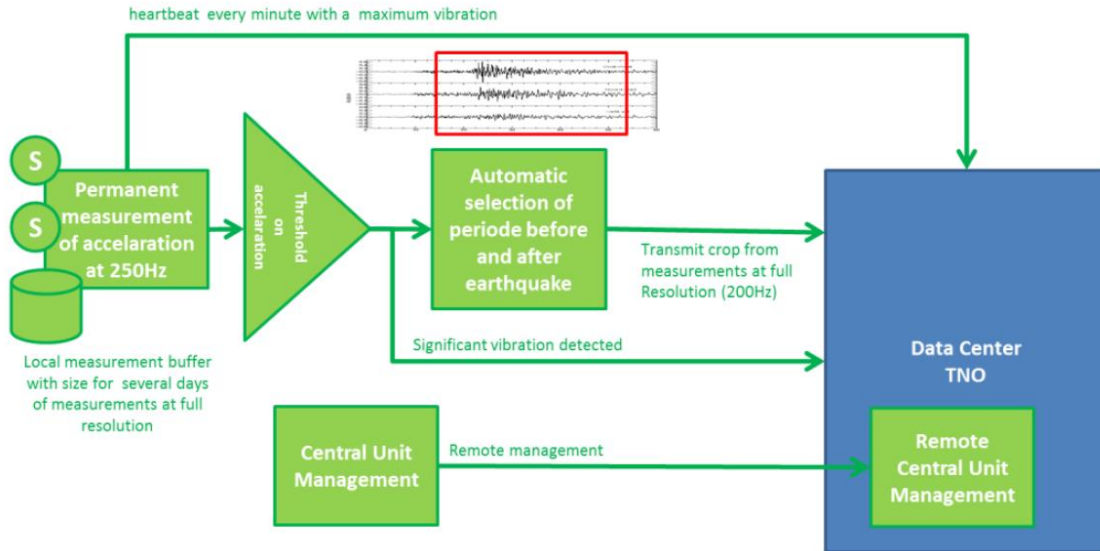
Figure 5.3 The sensors send their data event based when the vibration level exceeds a certain threshold and send a regular (every minute) heartbeat signal with a maximum vibration.
