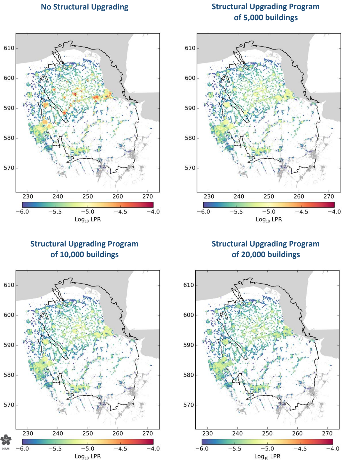
Figure 6. 12 Mean inside local personal risk maps for different upgrading plans between 2016 and 2021: (top left) no buildings upgrades, (top right) 5,000 building upgrades, (bottom left) 10,000 building upgrades, and (bottom right) 20,000 building upgrades. This assessment is for the 33 Bcm/annum production scenario for the period 2016 – 2021.
