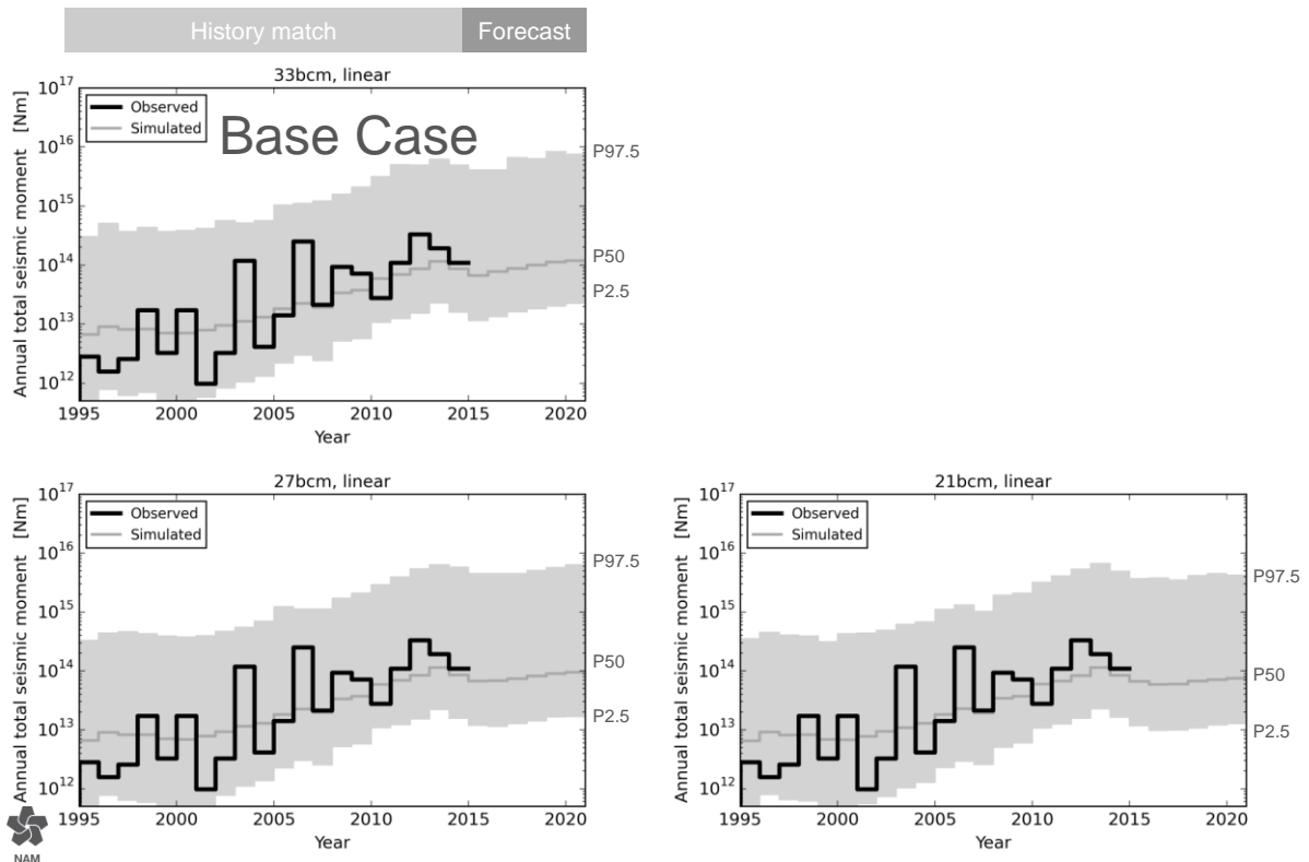
Figure 4.7 Total annual seismic moment time series including aftershocks.
