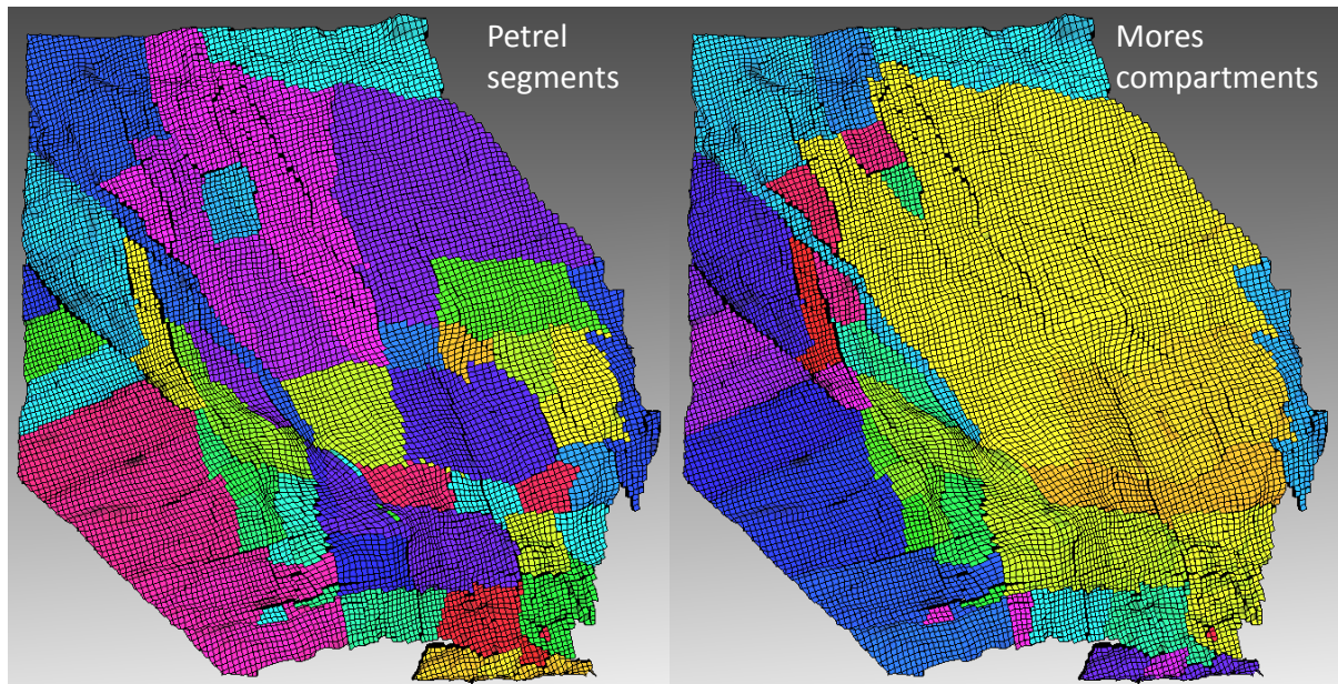
Figure A.3 Comparison between Petrel static model segments and Mores dynamic model compartments
