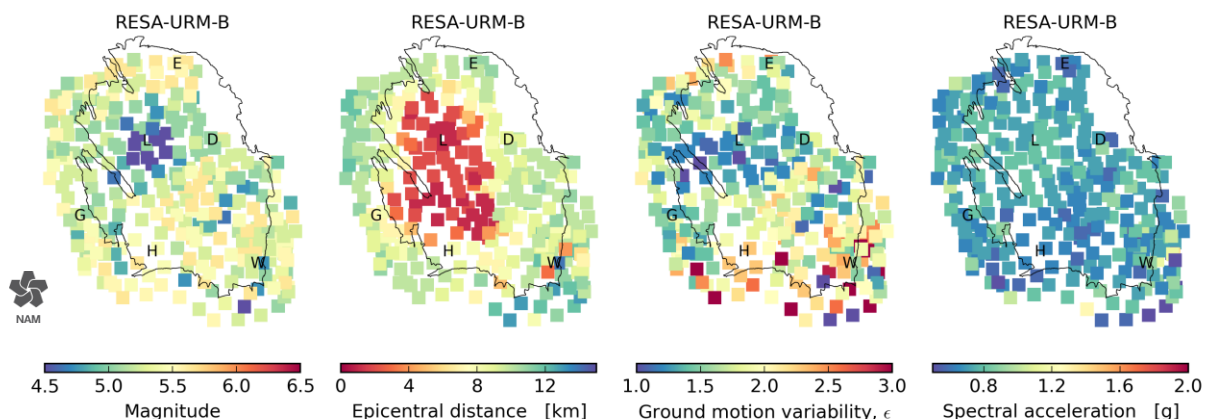
Figure 6.8 Risk disaggregation maps showing the modal contribution to ILPR at each map location for the period 2016 to 2021 under the 33 bcm/year production scenario and the base-case logic tree scenario.
