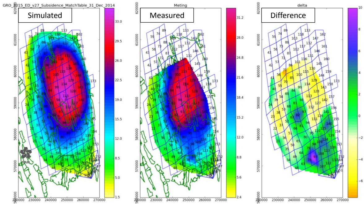
Figure 3.8 History match quality on subsidence using the proxy in Mores (scale is in cm). The high difference area in the south is associated with salt recovery. The mismatch in the south of the field is due to the subsidence caused by salt mining, which is not captured by the model.
