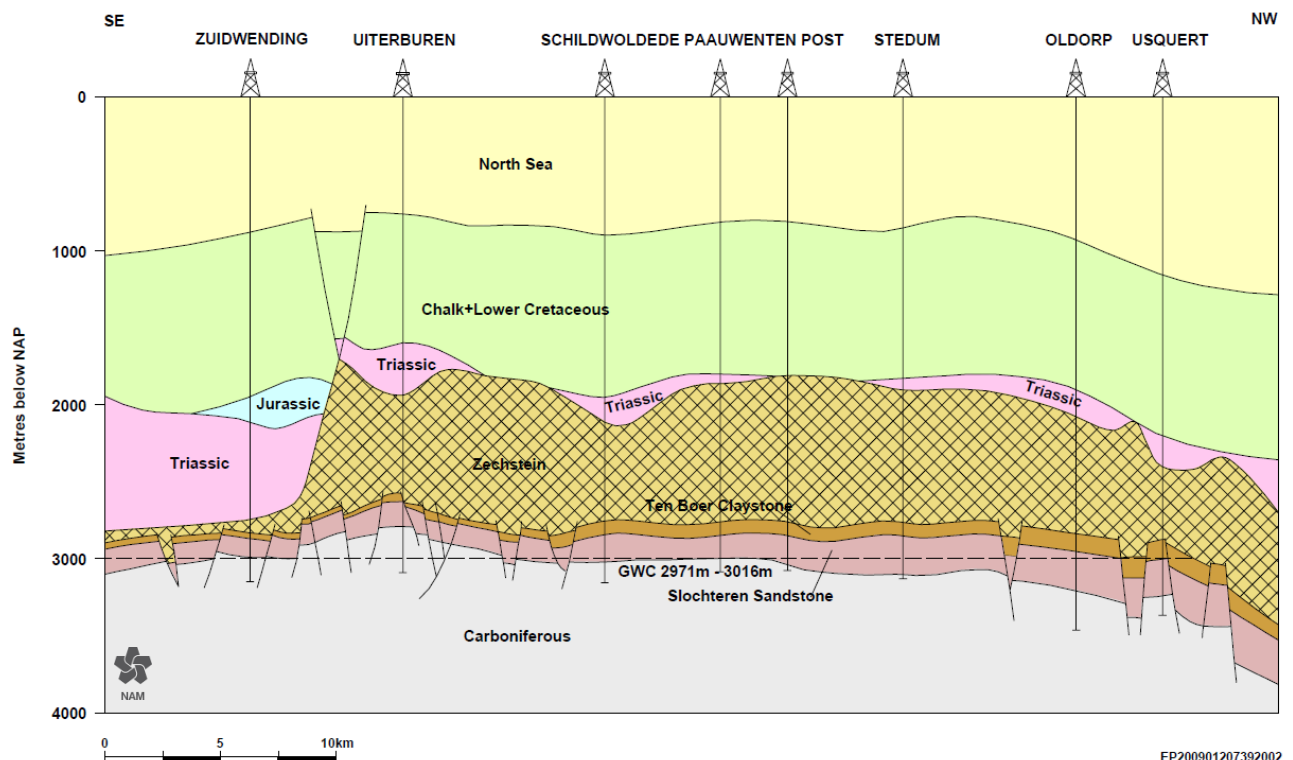
Figure 3.37 Simplified geological profile of the Groningen field. The thick Zechstein salt layers above the reservoir plays an important role in the transmission of seismic energy from the reservoir depth to the surface.
