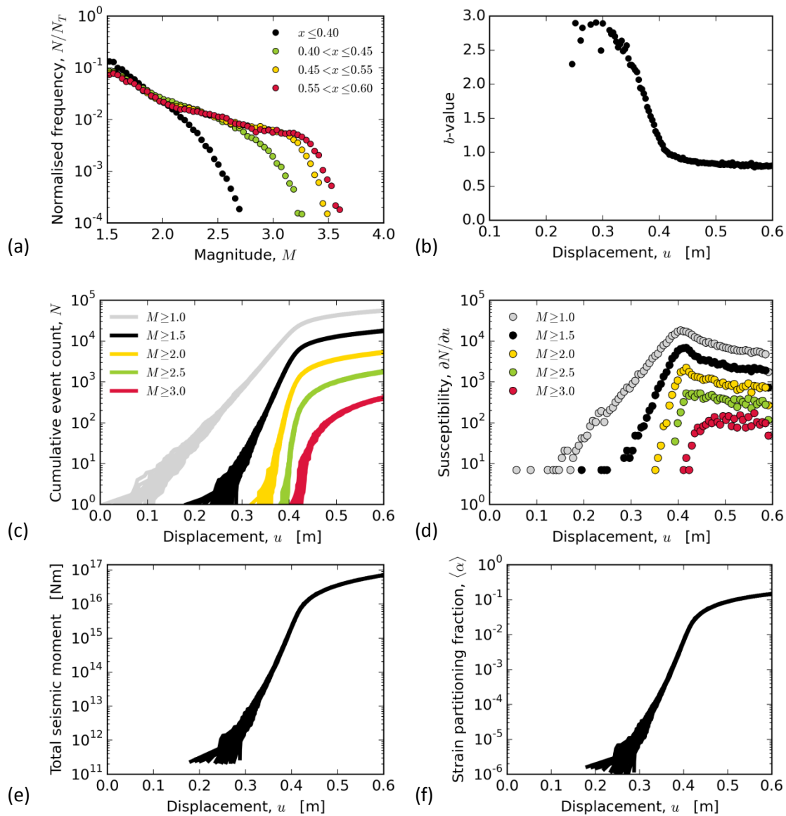
Figure 3.35 Example results obtained from a simple slider-block system with a physical extent of 60 km by 600 m comprising 10^5 blocks each about 20 by 20 m in size. (a) Frequency-magnitude distribution of slip events as it evolves with increasing relative displacement, x , of the plates with an upper bound influenced by the finite size of the system. (b) The trend of decreasing b -values with increasing initial relative displacement of the plates, u , before reaching some steady-state value. (c, d) The cumulative event numbers and the rate of event numbers show an exponential-like increase with increasing relative displacement of the plates until reaching some steady-state. (e, f) The total seismic moment and fraction of the total strain accommodated by slip (strain partitioning fraction) show an initial exponential-like increase with increasing relative displacement of the plates.
