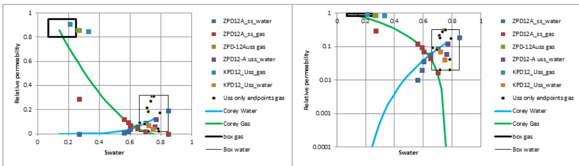
Figure A.6 Corey function fit for 14% porosity Swc (same as steady state experiment) to SCAL data on Groningen cores from steady state (ss) and unsteady state (uss) experiments
