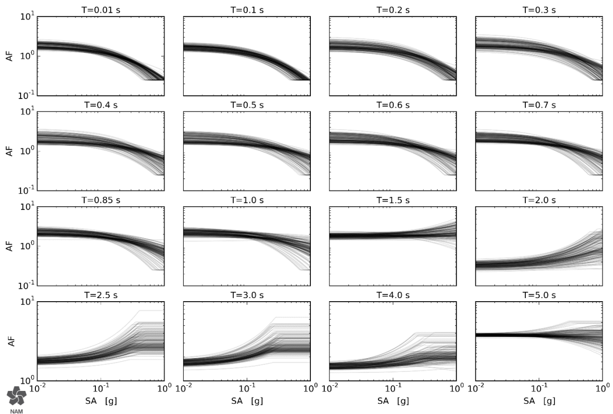
Figure 3.45 Non-linear site amplification factors (ratios of acceleration at the ground surface to acceleration at the NU_B horizon) for spectral accelerations at 16 oscillator periods
