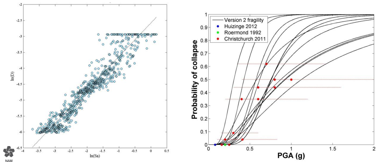
Figure 5.16 Results of nonlinear dynamic analyses and resulting fragility functions (the latter are herein defined in terms of PGA simply for the purpose of facilitating comparison with damage data from past earthquakes that have hit buildings with characteristics similar to those in Groningen)
