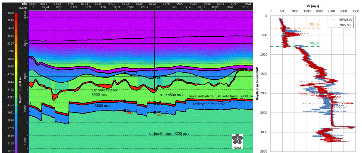
Figure 3.39 Left: P-wave model based on PSDM, DCAT and sonic logs S-wave model based on P – S sonic log relations per litho-stratigraphic unit. Figure 3.39 Right: Shear-wave velocity profiles from two deep borehole logs, indicating the location of the base of both the North Sea Supergroup Formation (NS_B) and the Upper North Sea Formation (NU_B) formations. The base of the Upper North Sea Formation NU_B horizon is seen as the interface between the hard rock and the softer and soil formations.
