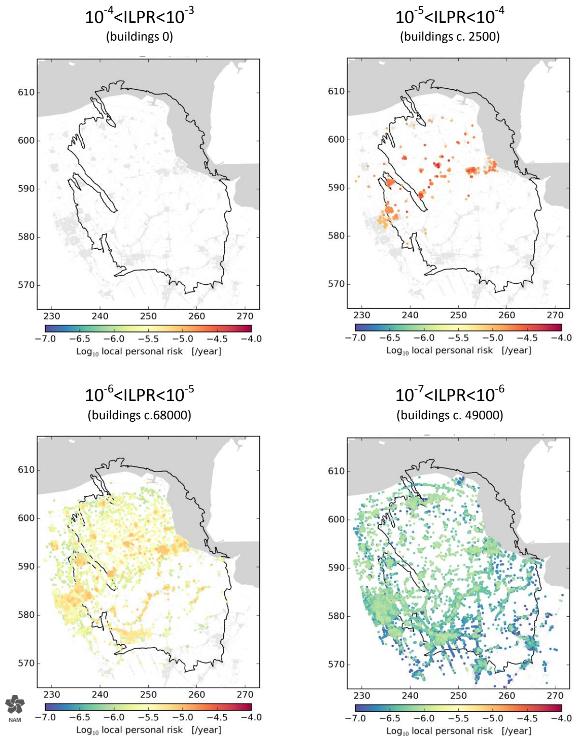
Figure 6.6 Mean inside local personal risk, ILPR for every individual building within four equal risk bands from 10^{-7} to 10^{-4} /year for the 5-year assessment period 2016 to 2021 under the 21 bcm production scenario. As Figure 6.5, except for the 21 bcm production scenario without structural upgrading.
