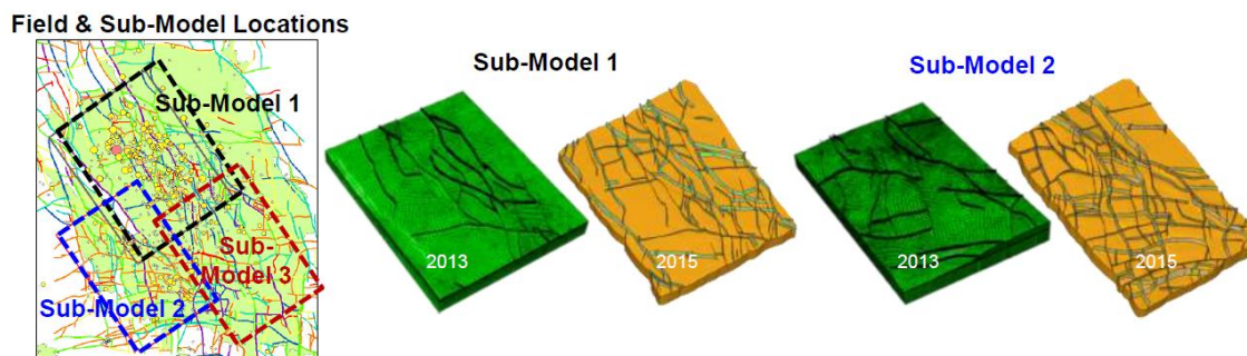
Figure 3.33 Large scale geomechanical model of the Groningen field. The additional complexity incorporated in this model since winningsplan 2013 in terms of faults and improved fault description with offsets is shown.
