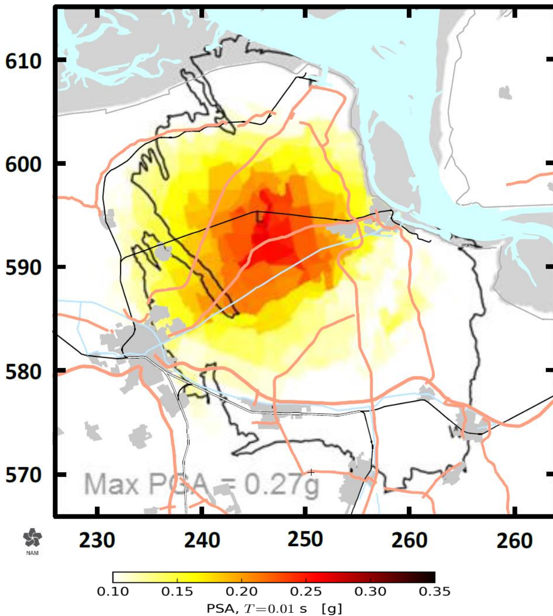
Figure 4.15 PGA hazard maps Period: 2016 – 2021, Production: 33 bcm/year, Compaction: Inversion, Activity Rate: V2.
