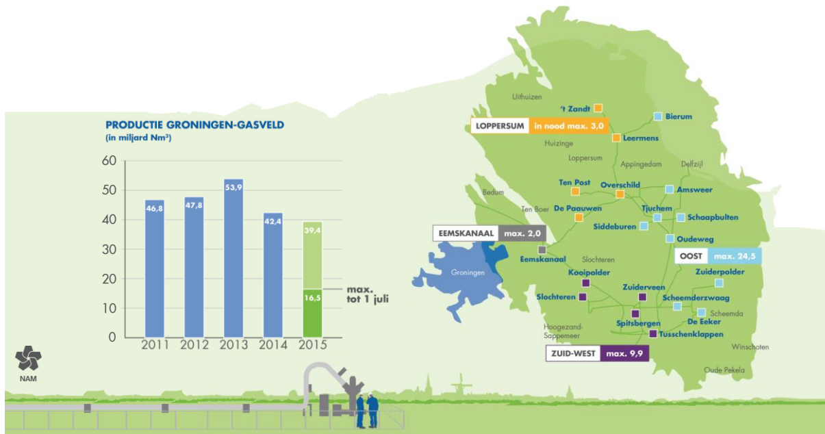
Figure 3.20 Grouping of the Groningen production clusters with production caps.
