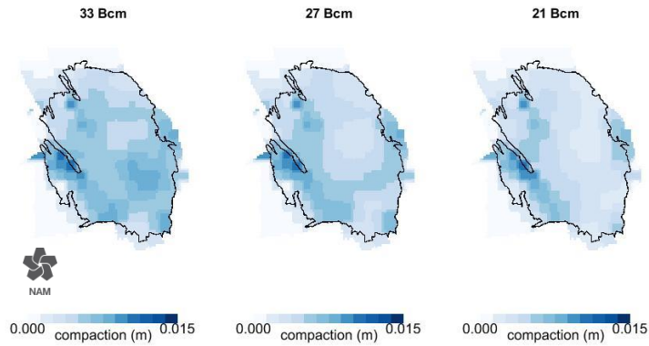
Figure 3.26 Compaction for the period 1-1-2016 to 1-1-2018 for three production scenarios using the linear compaction model
