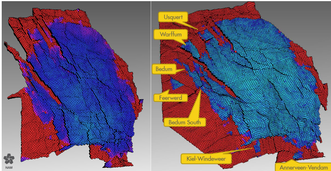
Figure 3.5 GFR2012 and GFR2015 grid boundary comparison. Small fields surrounding the Groningen field are located within this model area. Field names are indicated.
