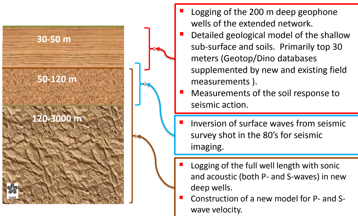
Figure 3.38 Rock column from the seismically active reservoir section to the surface (overburden), with the data gathering to improve our understanding of the progression of the seismic energy indicated in the boxes to the right.
