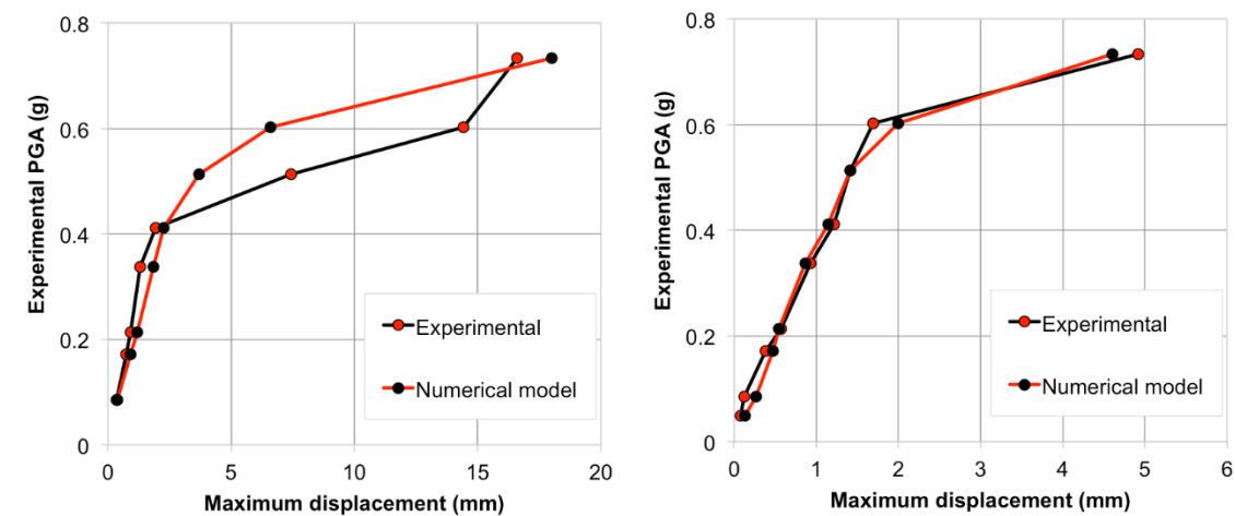
Figure 5.13 Comparisons of the predicted dynamic out-of-plane response of walls with the experimental results
