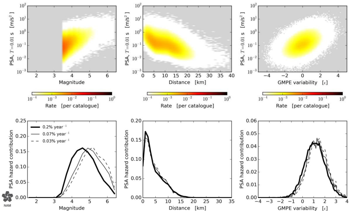
Figure 4.12 PGA hazard disaggregation (1) Period: 2016/1 – 2021/1, Production: 33 bcm/year, Compaction: Inversion, Activity Rate: V2, 3.5 \leq M \leq 6.5 , GMPE: V2 (Mea n) Location: Loppersum.
