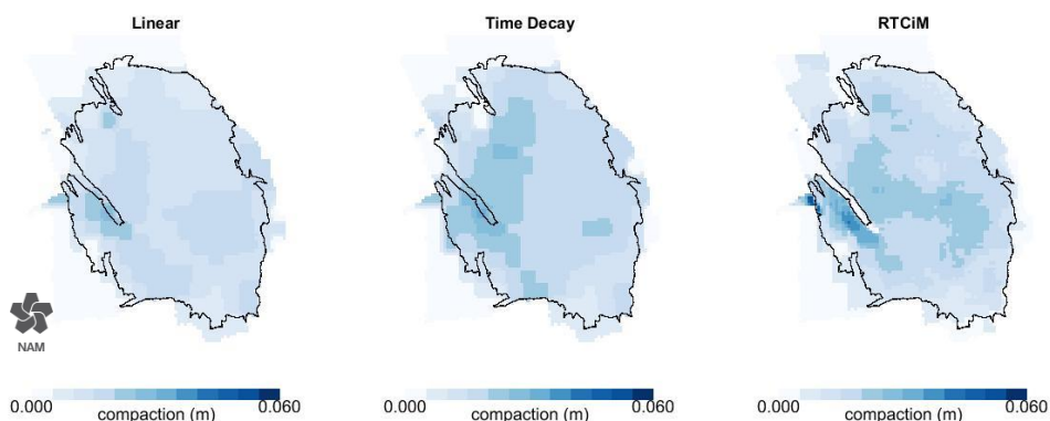
Figure 3.29 Compaction for the period 1-1-2016 to 1-1-2021 for the three compaction models (33 Bcm production scenario)
