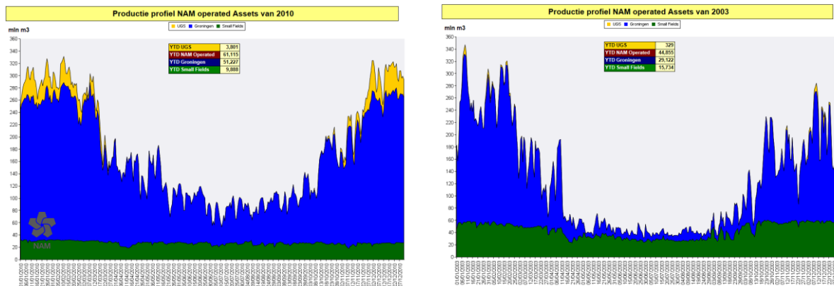
Figure 2.3 Intra-year production of NAM, 2003 versus 2010. (Small gas fields in green, Groningen main field in blue and the UGSs in yellow)
