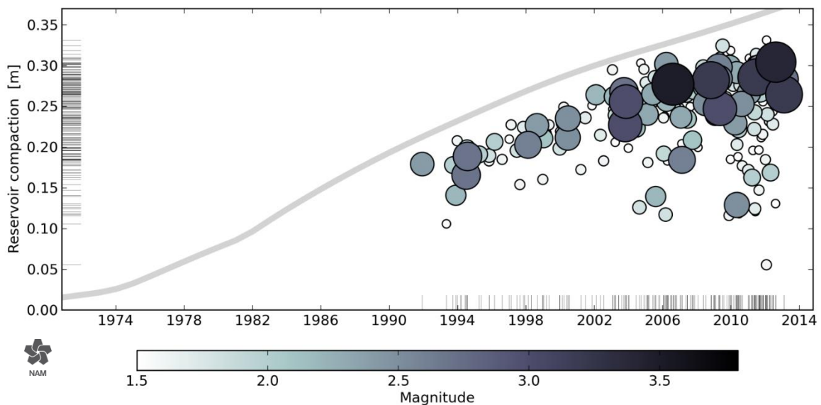
Figure 3.31 Time series of ML \geq 1.5 earthquake magnitudes versus reservoir compaction at the origin time and map location of each event.
