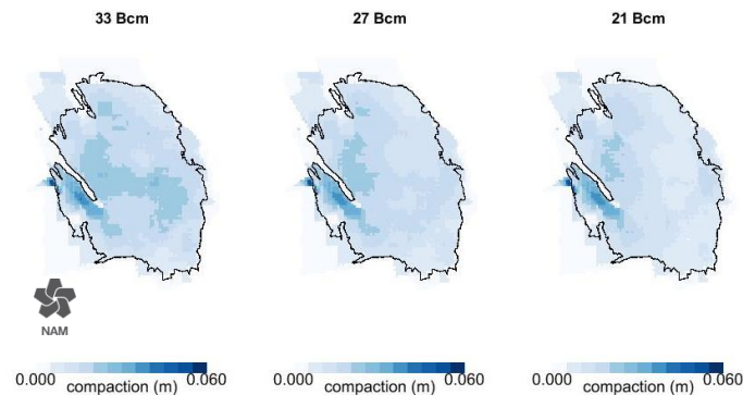
Figure 3.28 Impact of the production scenarios on the compaction using the RTCiM for the period 1-1-2016 to 1-1-2021
