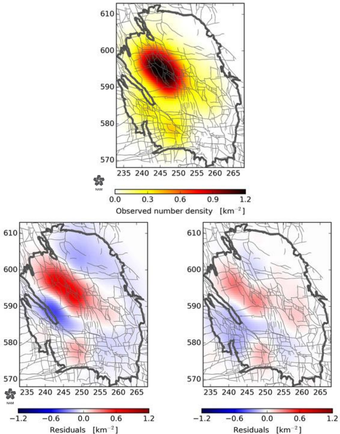
Figur 3.32 Observed and simulated seismic event density. Upper image shows the observed seismic event density. Lower images show the difference between the modeled and observed seismic event density for the two different versions of the activity rate model. Left result for the activity rate model based on compaction only and Right the impact when faults have also been taken into account.
