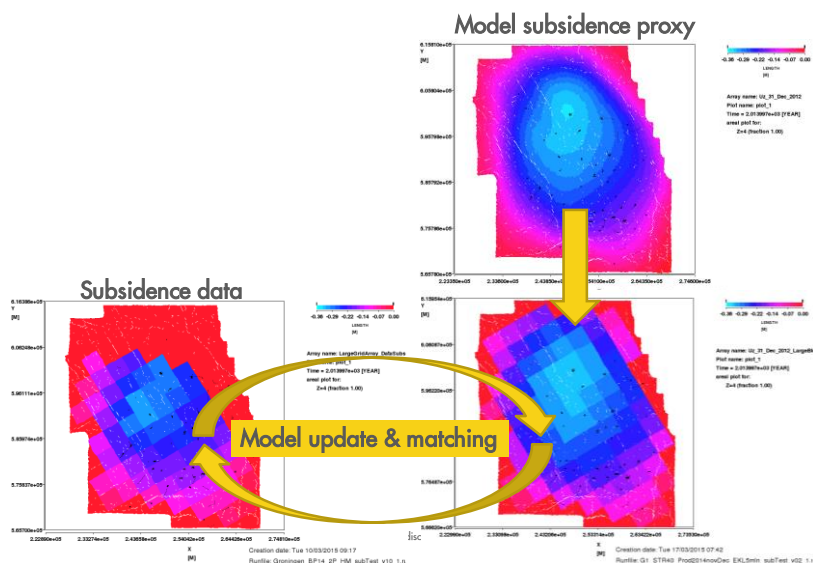
Figure A.2 Subsidence proxy implementation and workflow
