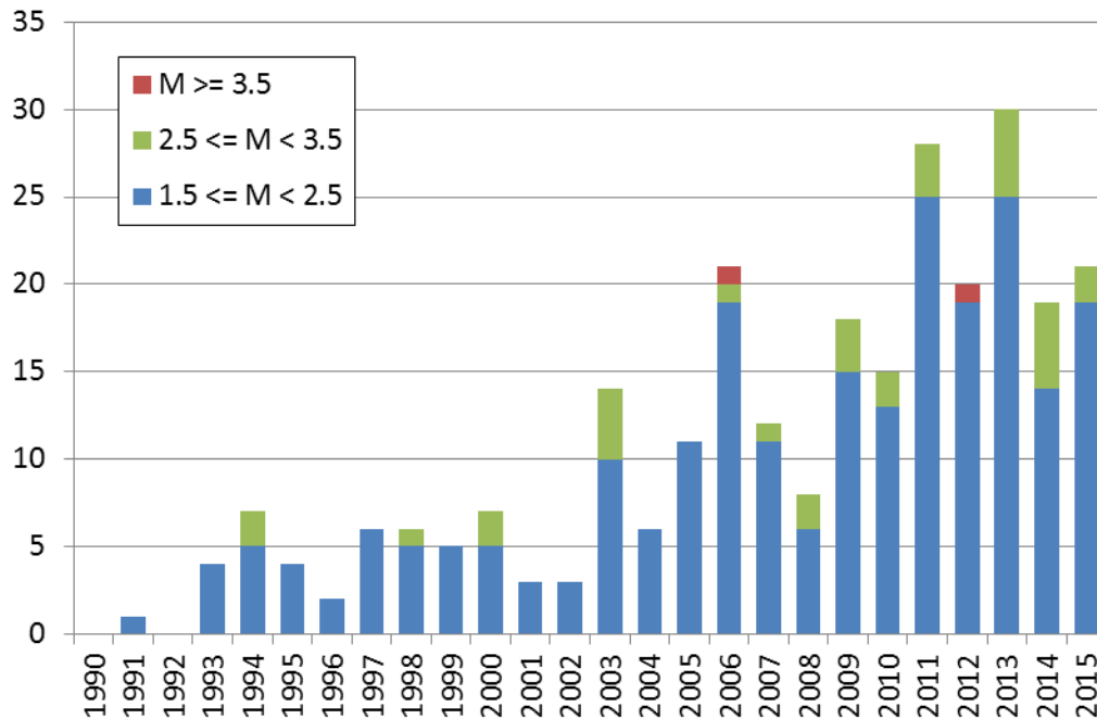
Figure 1. Number of events observed per year, categorized by magnitude (reported as local magnitude M_L ).
