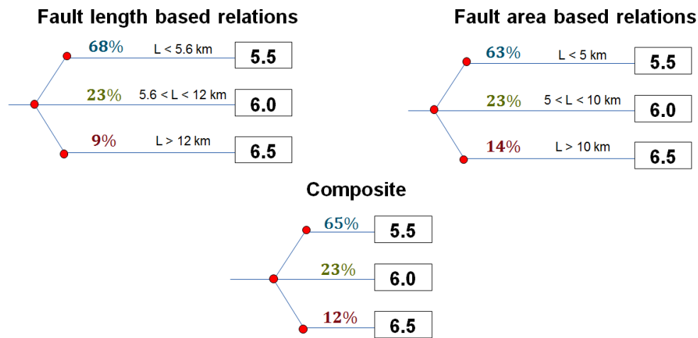
Figure 31. Few faults are large enough to host a large magnitude event, therefore the probability of applying a given truncation magnitude should depend on the relative abundance of faults capable of producing that magnitude event. Different scaling relationships will result in different relative likelihoods of the truncation magnitudes.
