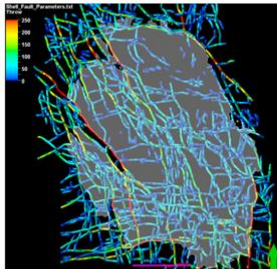
Figure 5. Fault throw (m) of all mapped faults used in the reservoir model. The faults with largest throw occur on the edges of the field (bounding faults).
