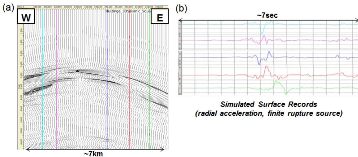
Figure B3. In the epicentral area there is significant variation in the waveform recording with small changes in observation location. (a) Seismic gather of many recordings along an east-west transect (b) A few highlighted recordings to demonstrate the large differences in waveforms.
