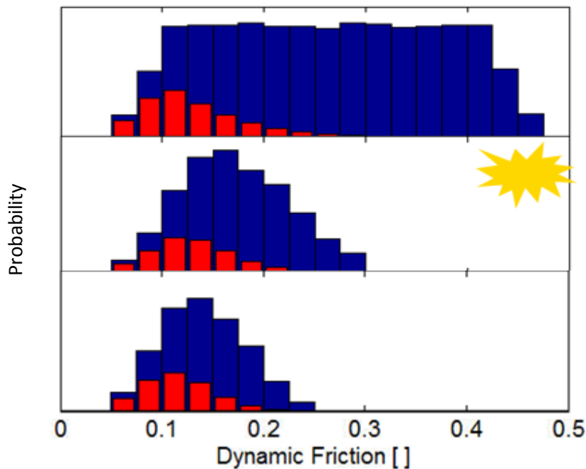
Figure 13. Three versions of assumed dynamic friction distributions. Distribution with the yellow star is the base case, base case distribution. The blue bars are the input assumed distribution for the Monte-Carlo analysis. For comparison, the red bars are the distributions of the cases that resulted in a stress drop during the Monte Carlo analysis.
