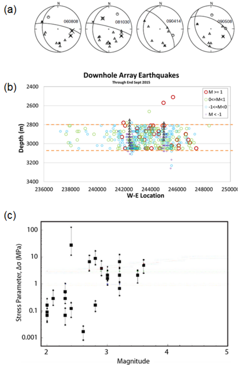
Figure 3. (a) Focal mechanisms indicate predominantly normal faulting with a small component of strike-slip motion (Kraaijipoel & Dost, 2013). (b) Location of events from the downhole array. Earthquakes are nucleating in the reservoir interval. The few events located out of the reservoir have large location errors and could easily fall within the reservoir interval (data posted to NAM platform) (c) Stress drops calculated from observed earthquake spectra range from \sim 0.1 -10 MPa (modified from Bommer et al, 2015a)
