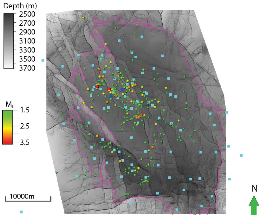
Figure 2. The current earthquake catalog for the Groningen field, through end of 2015. The field is outlined in pink and the depth map is the top of the Rotliegend reservoir. Current surface seismic stations are light blue squares and the downhole array locations are dark blue circles. Earthquake epicenters are circles and scaled/colored according to magnitude. Earthquake locations were obtained from the Royal Netherlands Meteorological Institute's website (KNMI, 2016). Lateral error in the location is estimated by KNMI to be ~1 km, while depth is assigned to be 3 km – within the reservoir.
