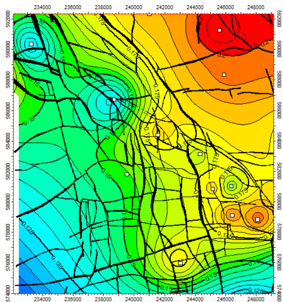
Figure 11 Porosity [fraction] for the Upper Slochteren Sandstone Formation is shown for reservoir layers 2 and 3.
