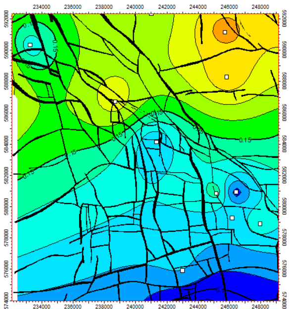
Figure 12 Porosity [fraction] for the Upper Slochteren Sandstone Formation reservoir layer 1 and the Lower Slochteren Formation reservoir layers 2.
