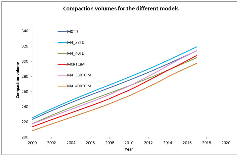
Figure 27 Total compaction volume for Winningsplan (Dark blue and Red, M0) and the two sub-surface models Model 1 (Green and Brown, 40) and Model 2 (Light blue and Purple, 38) for the EKL base case production of 8 mln m 3 /day average, calculated with both the Time-decay (TD) and RTCiM compaction models.
