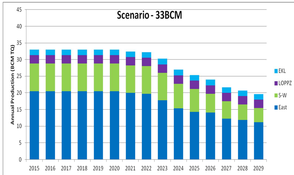
Figure 8 An indicative gas production schedule for scenario II. Production is kept below 33.0 Bcm, until the natural decline of the production from the field sets in. No additional development wells are drilled.
