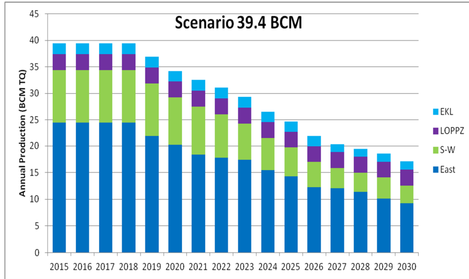
Figure 7 An indicative gas production schedule for scenario I. Production is kept below 39.4 Bcm, until the natural decline of the production from the field sets in. No additional development wells are drilled.
