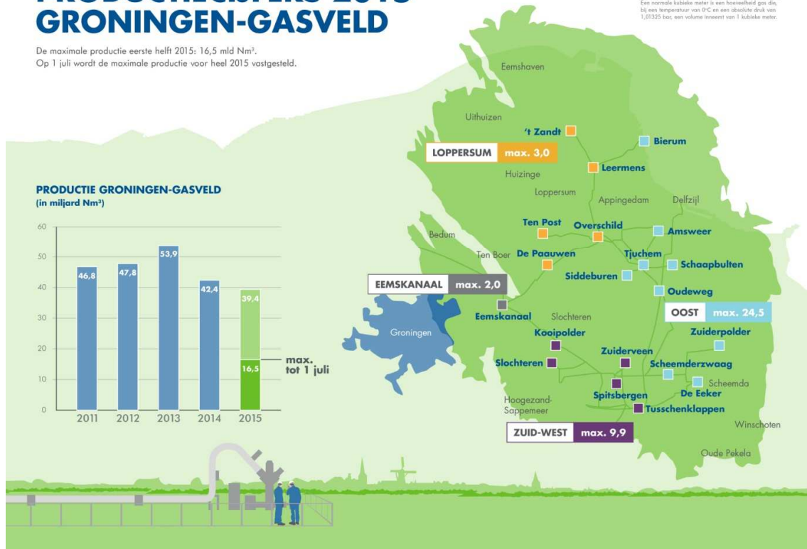
Figure 10 Spatial and temporal production caps have been imposed. Production caps have been imposed on 5 groups of production clusters. Additionally, the production has been capped for the first and second half of 2015.
