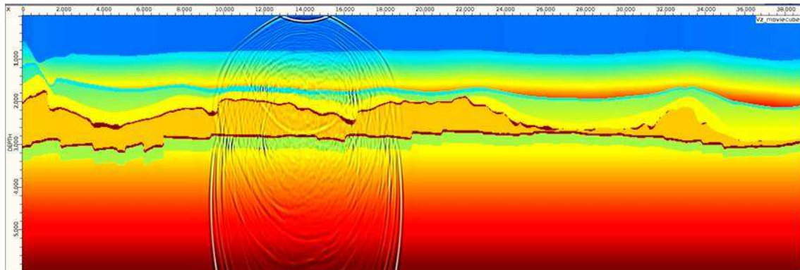
Figure 17 Results of a simulation of earthquake waves moving towards the surface.
