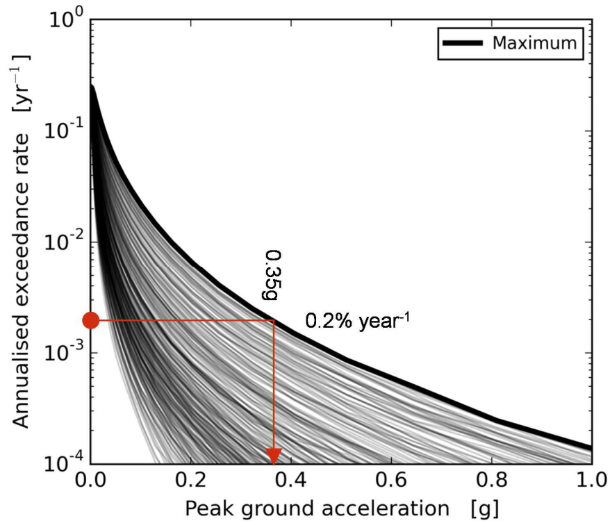
Figure 19 Annual exceedance rate for peak ground acceleration at different locations in the field. This was assessed for the period 2016 – 2021 and the 39.4 Bcm production scenario. Each line corresponds to a location in the field. The bold line indicates the maximum PGA in the field for a given exceedance level (bounding envelope).
