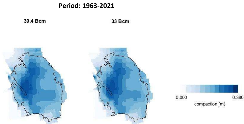
Figure 12 Cumulative compaction from the start of production to 2021 for both production scenarios based on the inversion of levelling data (linear compaction model)
