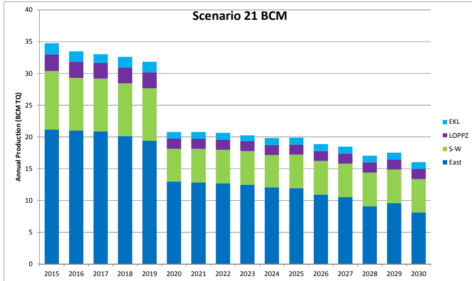
Figure 9 An indicative gas production schedule for Scenario III. Production is kept below 33 Bcm from 2016 onwards and further reduced to 21.0 Bcm from 1-1-2020 (as soon as additional gas blending capacity is available), until the natural decline of the production from the field sets in. No additional development wells are drilled.
