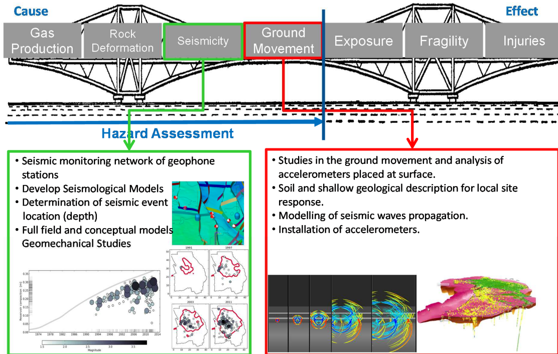
Figure 15 The causal bridge continues with seismicity resulting from the deformation of reservoir rock and the prediction of the ground motion (PGA).
