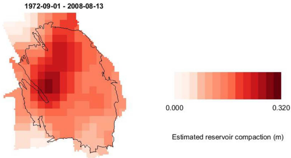
Figure 11 Example of a compaction grid calculated from the levelling surveys for the period 1972-2008.
