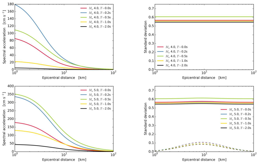
Figure 16 Variation in the median GMPE with epi-central distance (left) and the associated variability (right) for a (top row) M4.0 and (bottom row) M5.0
