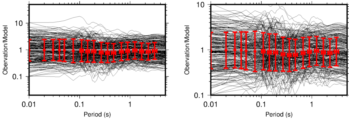
Figure 9.8 Residual misfit between the simulations – modified to use stress parameter and \kappa directly inverted from the corresponding FAS – and the V1 database.
