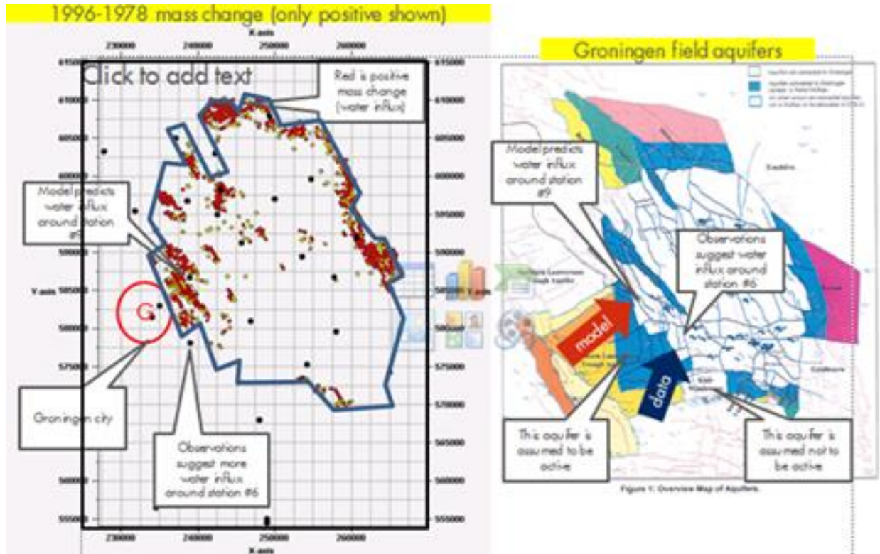
Figure 6.6 Gravity survey to be used in AHM.
