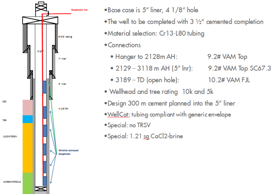
Figure 3.15 Well design for the two permanent geophone wells in the Loppersum Area
