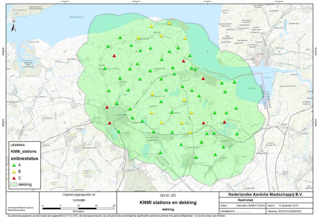
Figure 3.5 Extension of the shallow borehole geophone network with 69 locations. The locations indicated by A have a stable data connection; B: have an instable data connection and C: no data connection. The data is stored at the station location.
